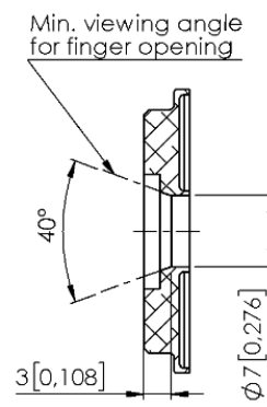
SECTION G-G
